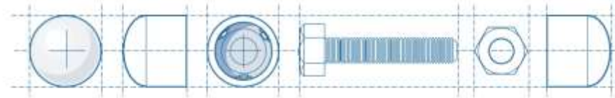
Metric Bolt Cap overall dimensions
